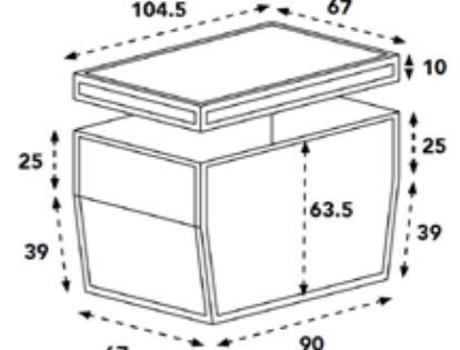
Flightcase Trike
