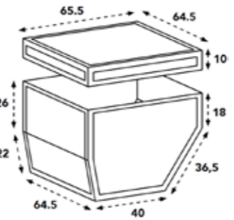
Flightcase short
