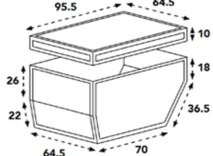
Flightcase Long
